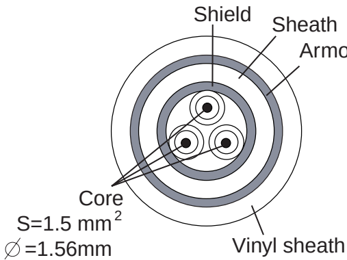
TPYCYS-1.5 sectional view
