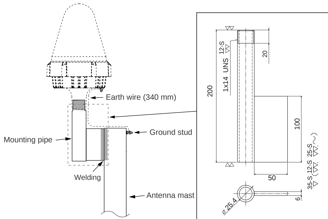
Mounting pipe and antenna mast
