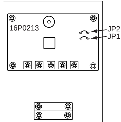
Alarm unit IC-306
