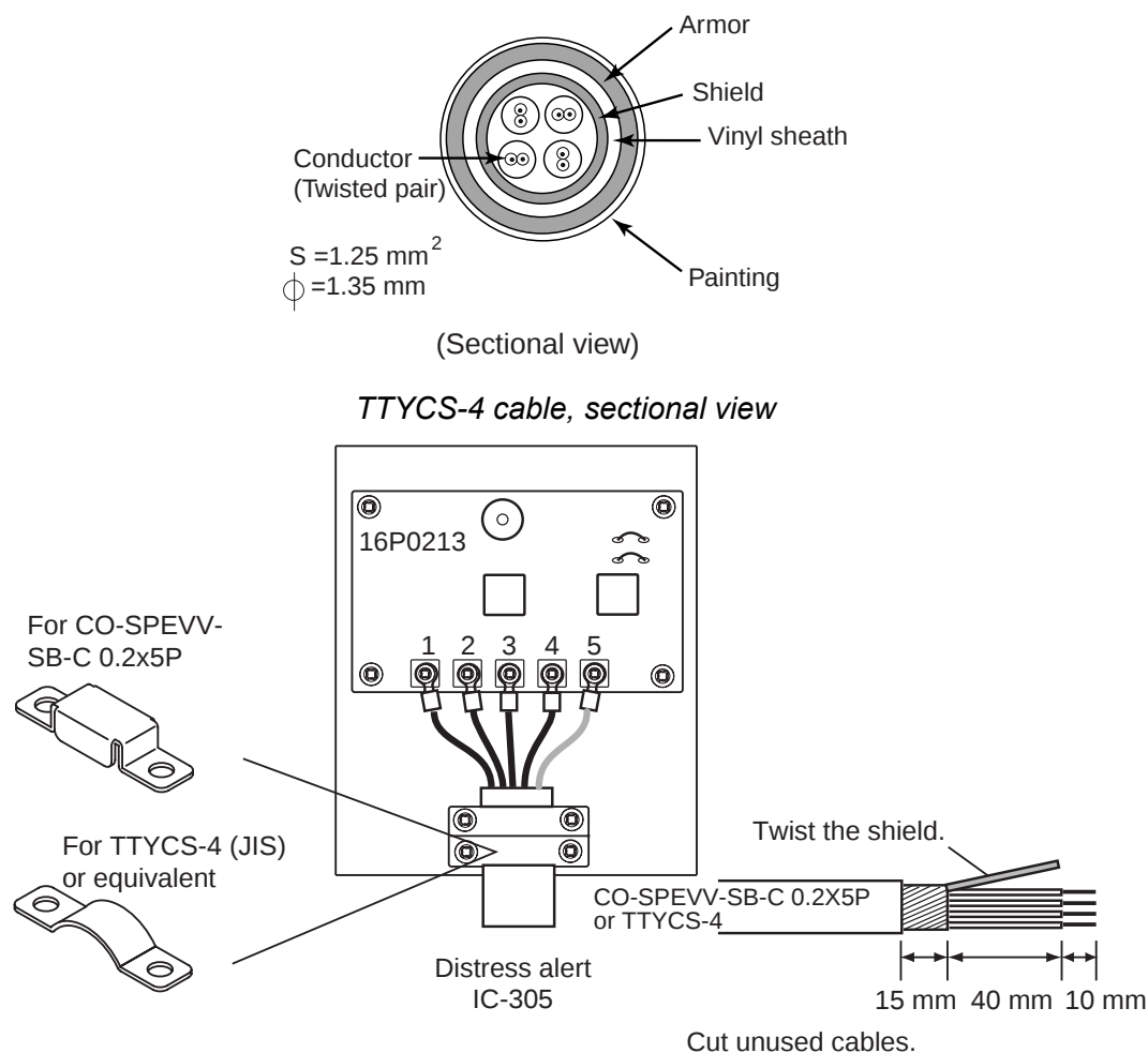
Wiring of distress alert IC-305
