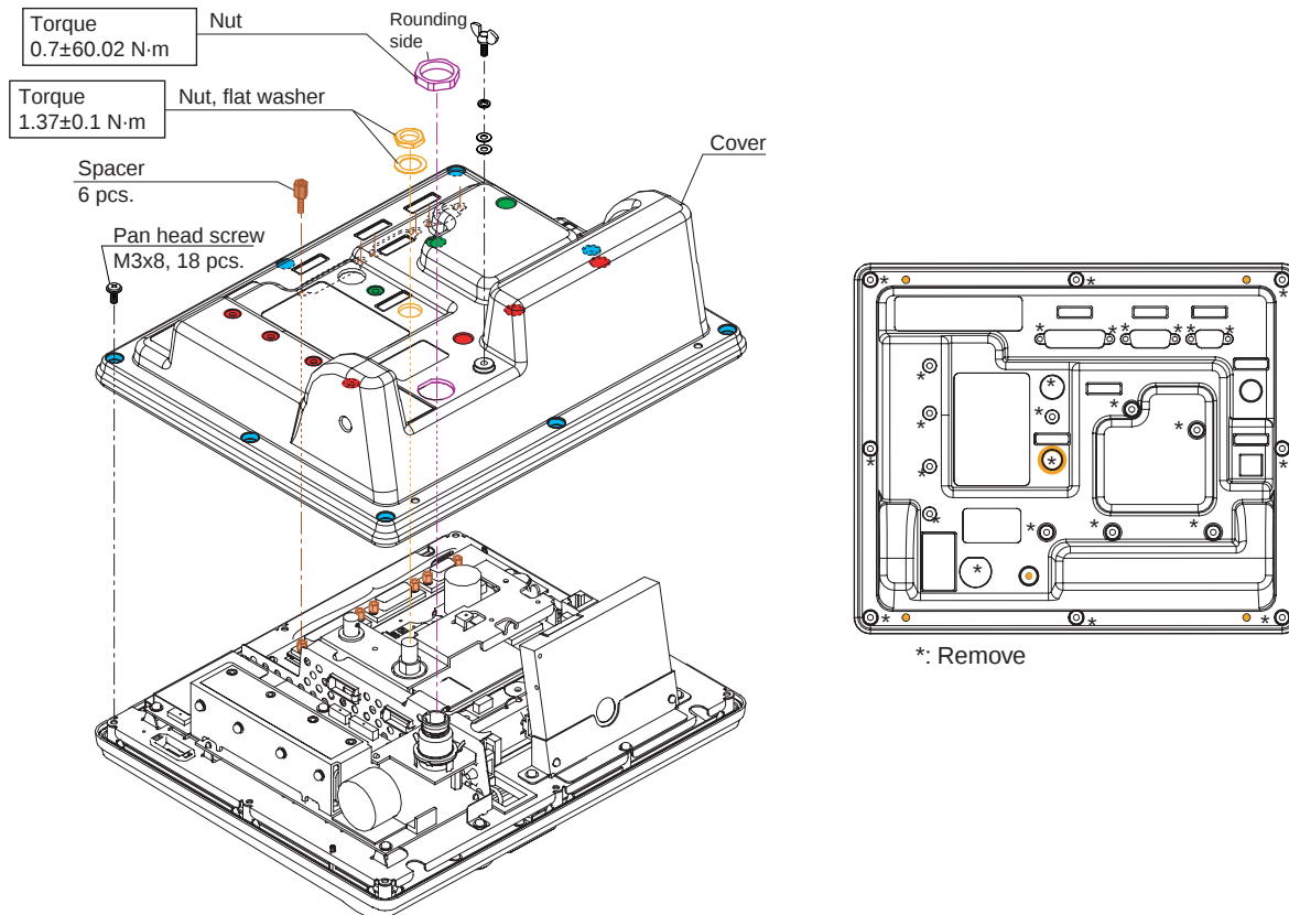
Terminal unit, cover removed
