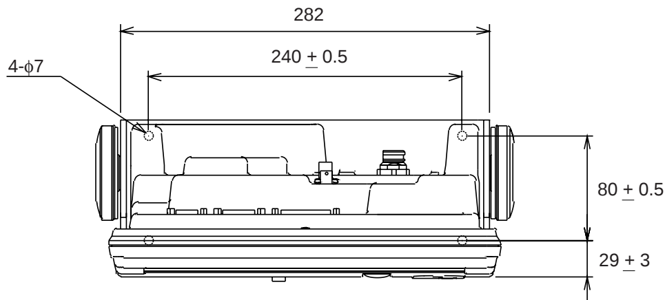
Terminal unit, tabletop mounting
