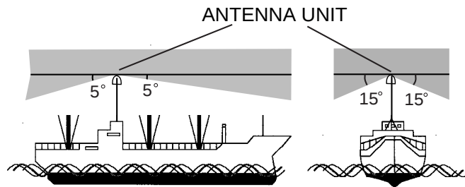
Antenna unit mounting location
