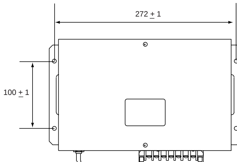
AC/DC power supply unit, dimensions
